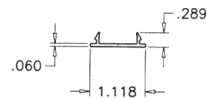
T4 HEAD COVER
