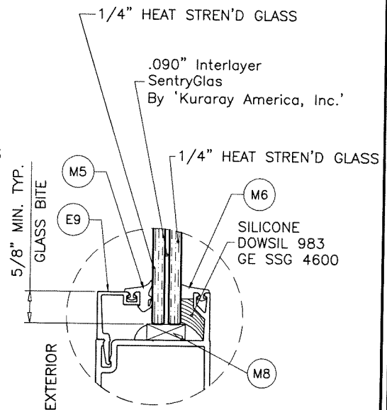
GLASS TYPE 'B.1' 9/16" OVERALL LAM. GLASS
