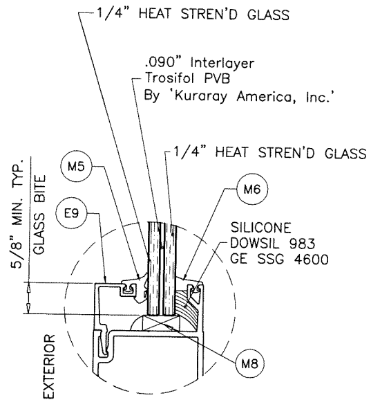
GLASS TYPE 'A.1' 9/16" OVERALL LAM. GLASS
