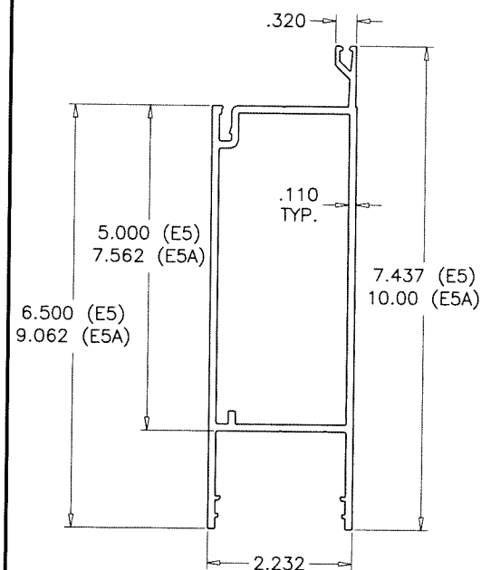
E5 STD. BOTTOM RAIL E5A HI-PROFILE BOTTOM RAIL
