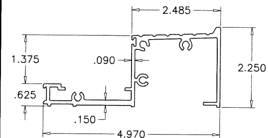
(E2B) HIGH THRESHOLD APPR'D FOR WATER RESISTANCE
