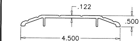
(E2A) SADDLE THRESHOLD ES9015
