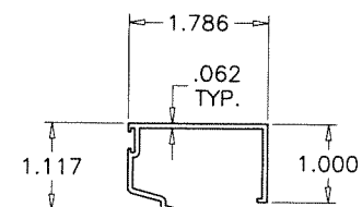
T9 TRANSOM GLASS STOP S-8000
