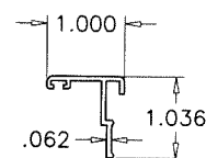
E5 STD. BOTTOM RAIL E5A HI-PROFILE BOTTOM RAIL
