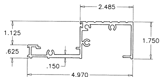
(E2D) MEDIUM THRESHOLD NOT APPR'D FOR WATER RESISTANCE
