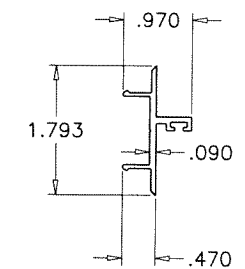
(E3.2) NARROW JAMB DOOR STOP
