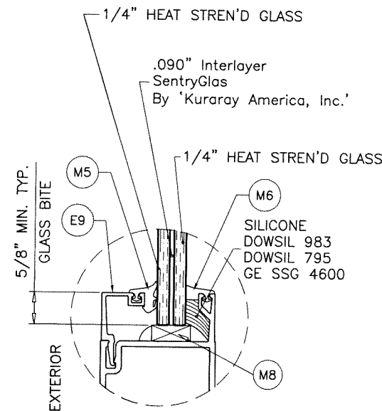
GLASS TYPE 'B' 9/16" OVERALL LAM. GLASS
