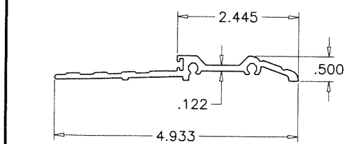
(E2) STD. THRESHOLD ES9014
