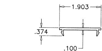
(E2C) THRESHOLD COVER ES9027
