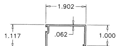
T9A TRANSOM GLASS STOP S-8000T
