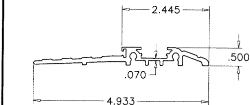
(E2.1) ALT. STANDARD THRESHOLD
