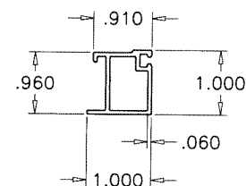
T3 TRANSOM GLASS STOP
