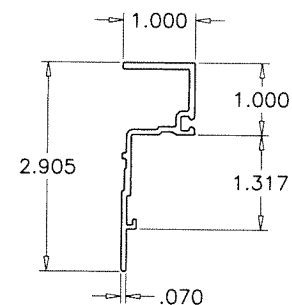
T2 TRANSOM ADAPTER
