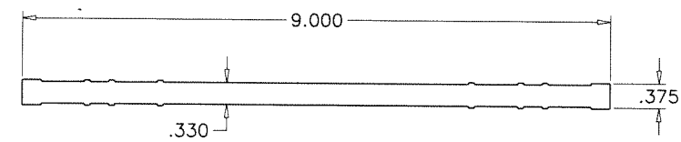
(E13) HINGE BACKUP PLATE
