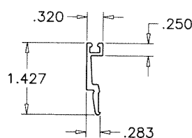
E9.1 GLASS STOP (INSUL. LAM. GLASS)
